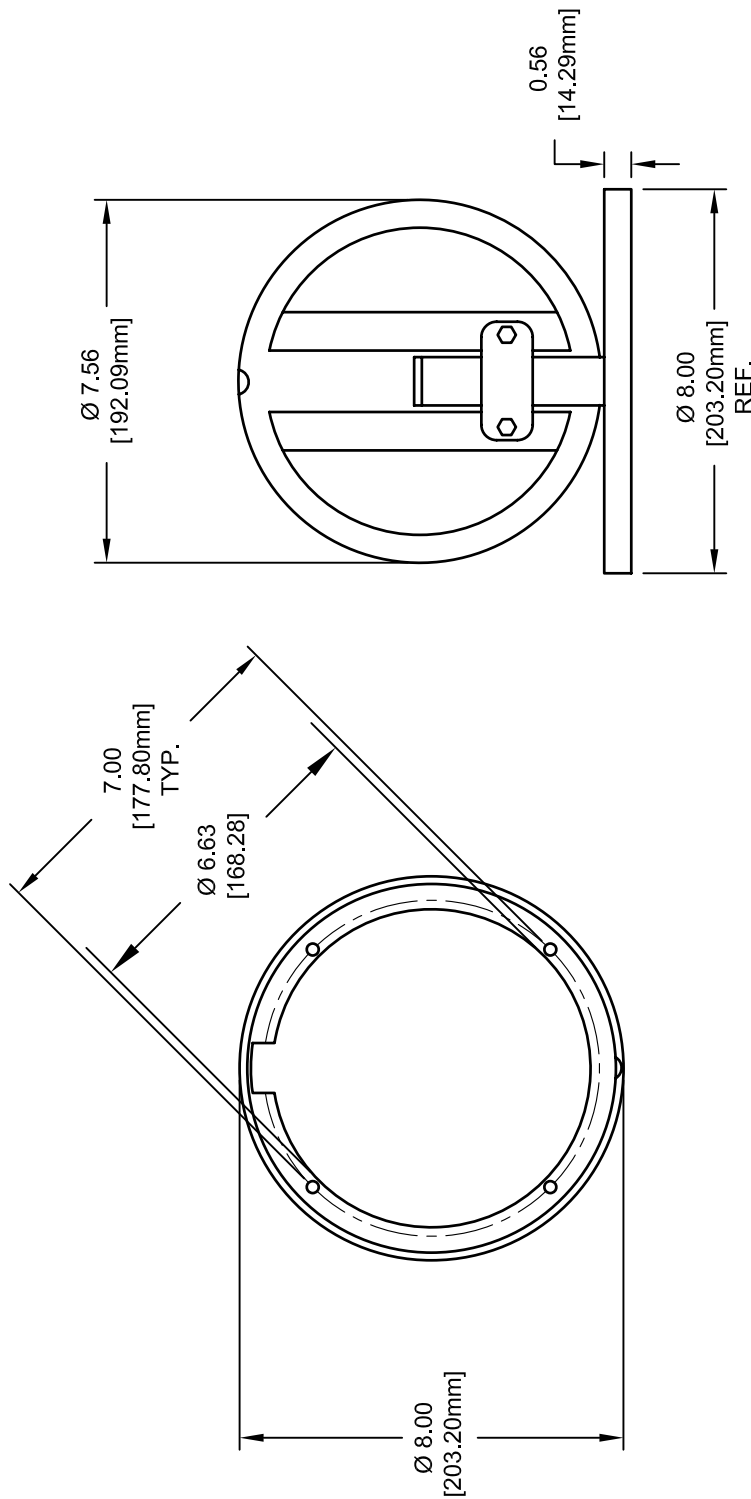
TOP VIEW WITHOUT COVER
