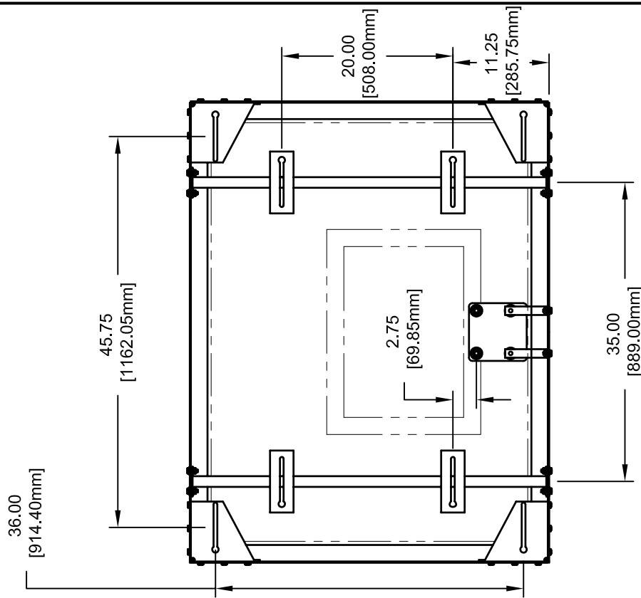
REAR VIEW
