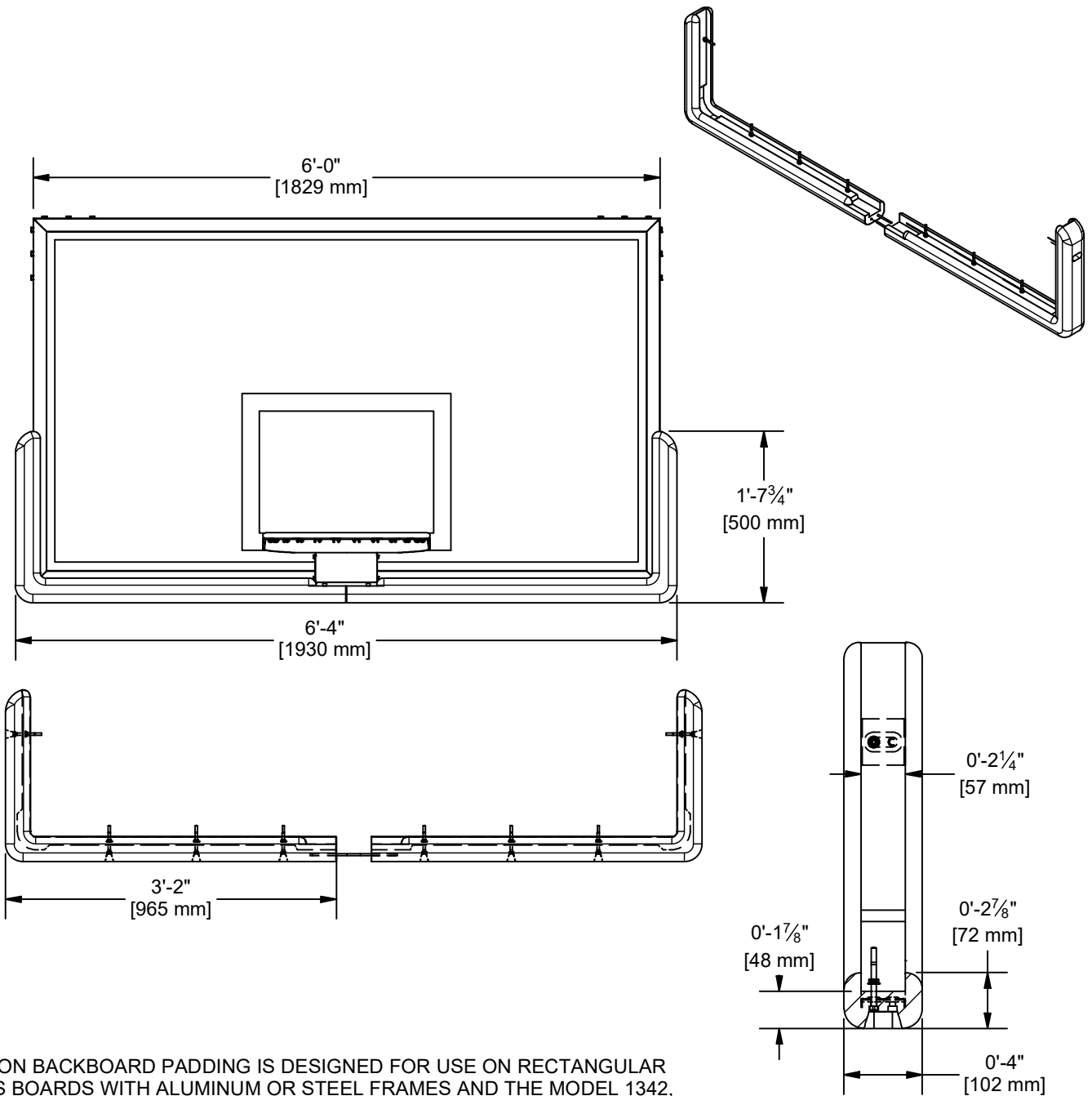
CROSS SECTION
