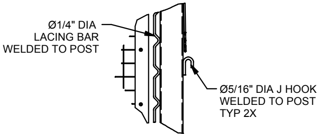
DETAIL A
