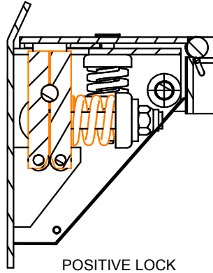
POSITIVE LOCK DETENT MECHANISM
