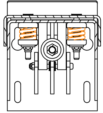
DUAL RETURN SPRINGS
