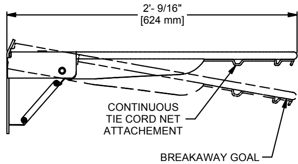
BREAKAWAY GOAL
