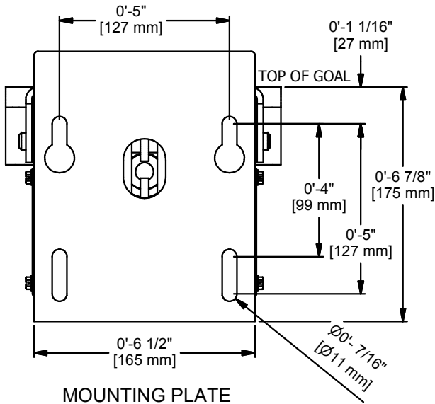
MOUNTING PLATE
