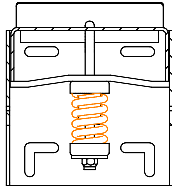
BREAKAWAY SPRING
