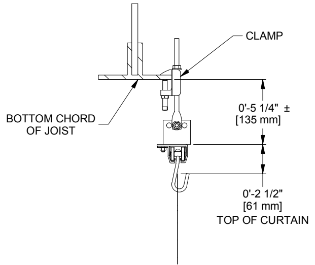
JOIST ATTACHMENT DETAIL
