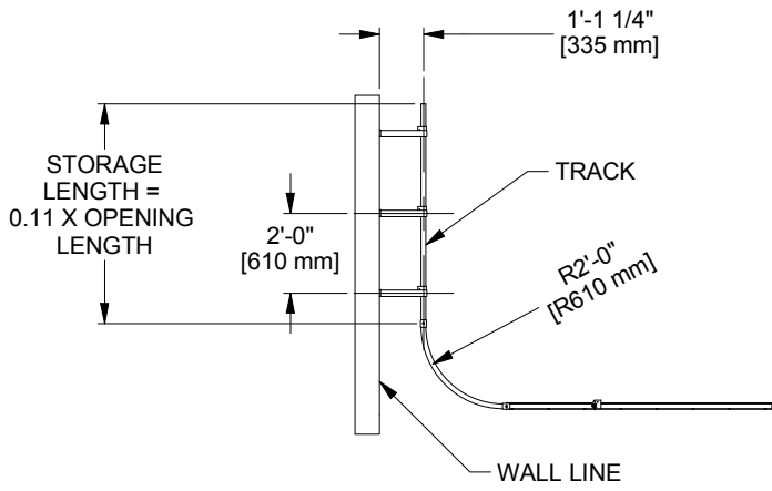
CURVE AND STACK DETAIL (OPTIONAL)
